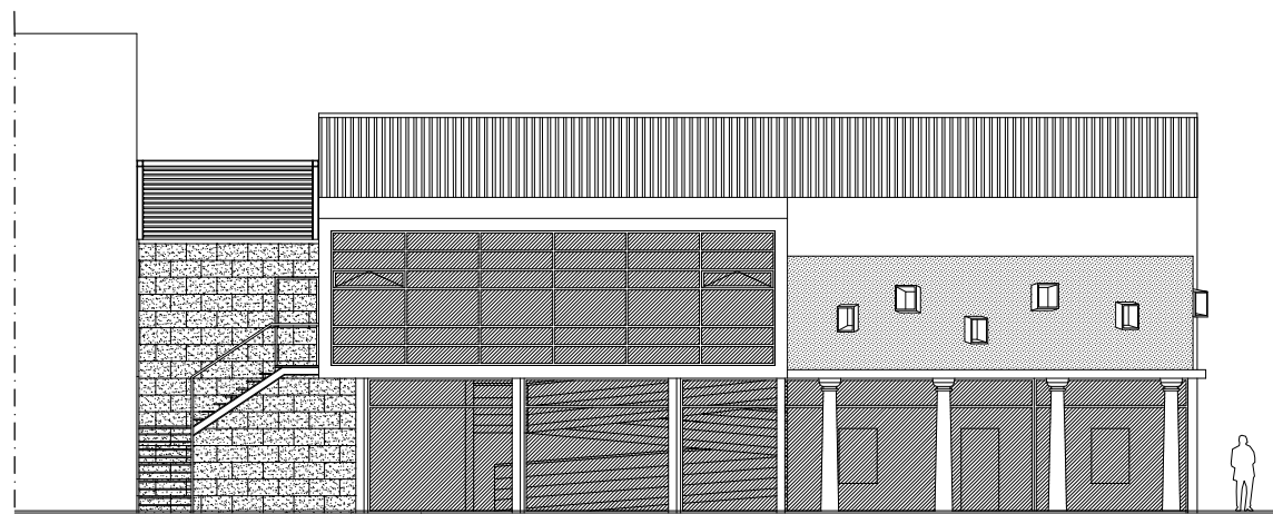
Façana Principal
